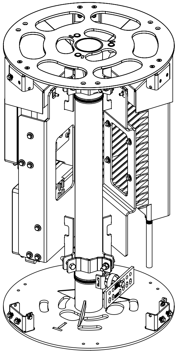
STEP 3 •POLETOP 18" AFTER REMOVING TWO BRACKETS
