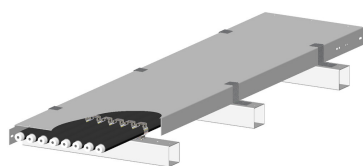
Rooftop Coaxial Cable Bridge Kit, for 12 coaxial cable runs,12-gauge cover
